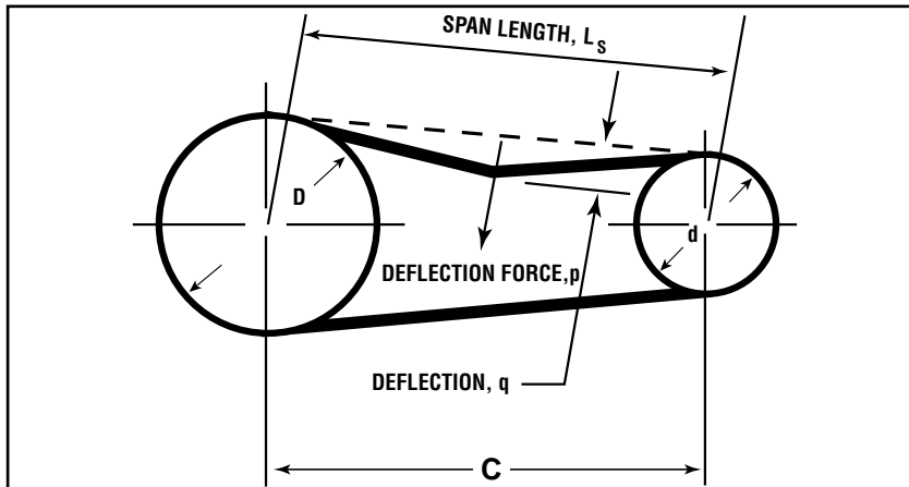
Figure 26 — BELT DEFLECTION DIAGRAM
