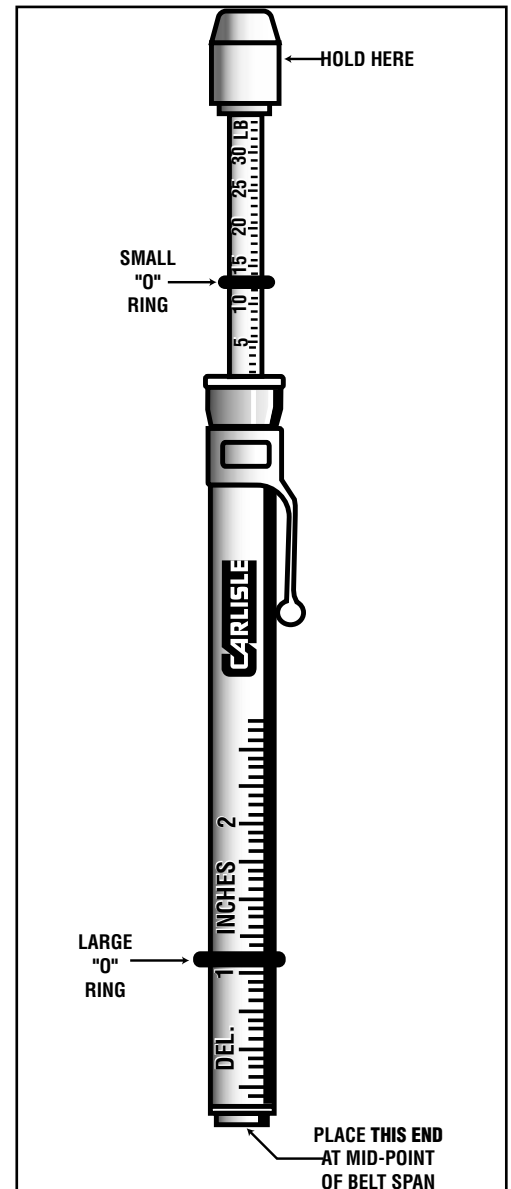
Figure 28 V-BELT TENSIONER (Part No. 102761)
