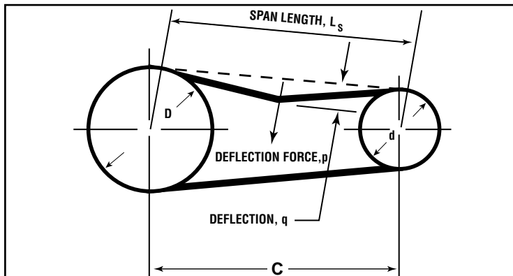
Figure 1 MEASURING DEFLECTION FORCE
