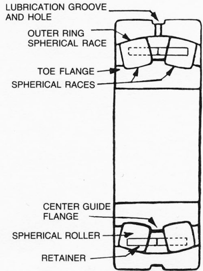
SPHERICAL ROLLER BEARING
