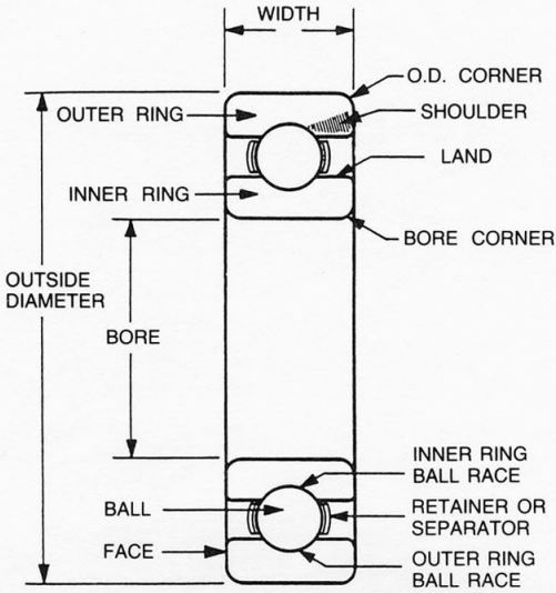
BALL BEARING
