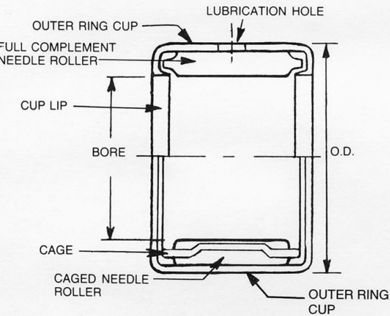
DRAWN CUP NEEDLE BEARING
