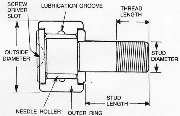
CAM FOLLOWER
